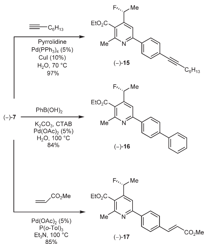
Scheme 5. Synthesis of pyridines (–)-15 to (–)-17.
