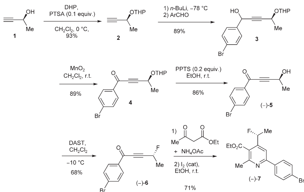
Scheme 2. Synthesis of pyridine (–)-7.
