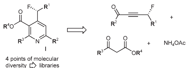
Scheme 1. Retrosynthetic analysis for the preparation of type I pyridines.
