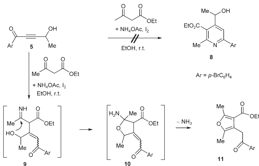
Scheme 3. Synthesis of furan 11 .
