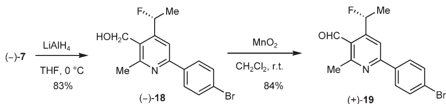
Scheme 6. Synthesis of pyridines (–)-18 and (+)-19.
