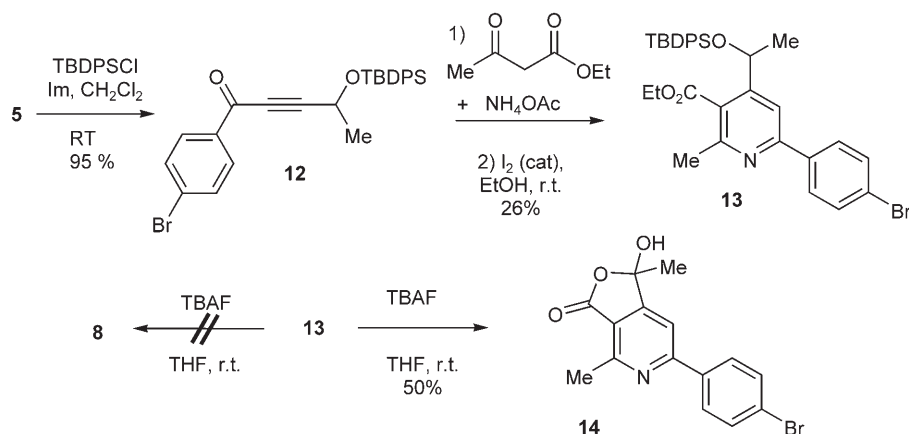
Scheme 4. Synthesis of pyridine lactol 14 .
